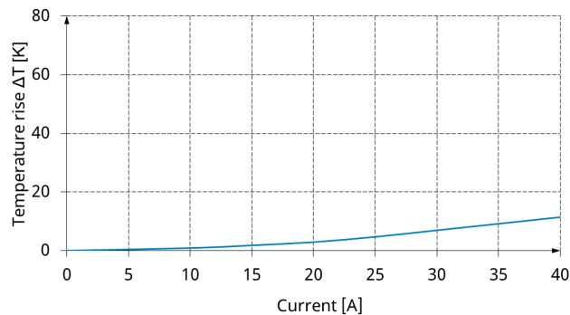
Current Rating
