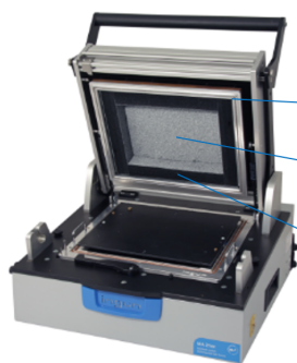
Top RF chamber Conductive surface (light grey) Non-conductive surface (anthracite)
