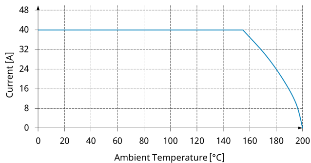
Current Derating
