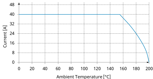
Current Derating
