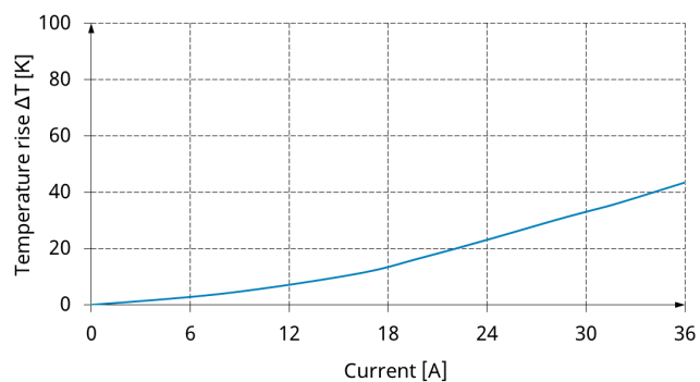
Current Rating
