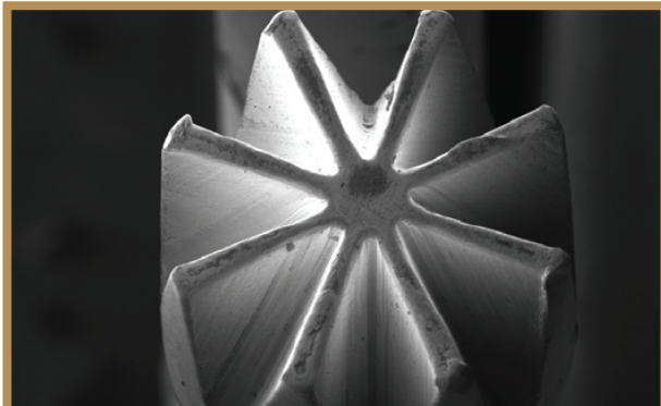
Tip Style 79-Star (Ø 0,90 mm, 8 contacting edges) Number of contacts: 0
