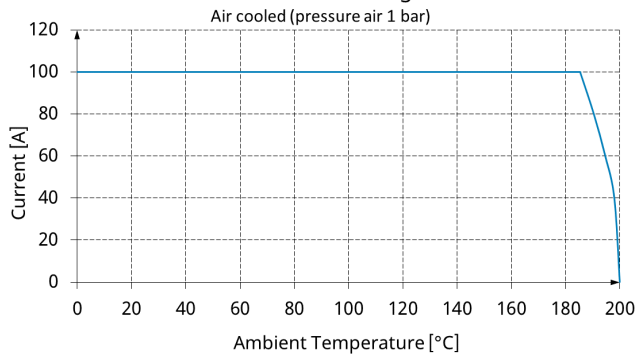
Current Derating
