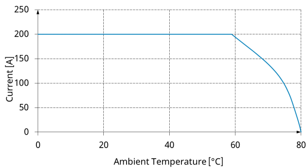
Current Derating
