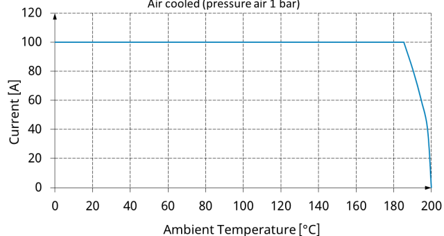
Current Derating Air cooled (pressure air 1 bar)
