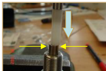
7. Press in the spare parts vertically until friction bearing flush with head of marking unit. Secure the marking head vertically in place to avoid axial strains of the gear motor.
